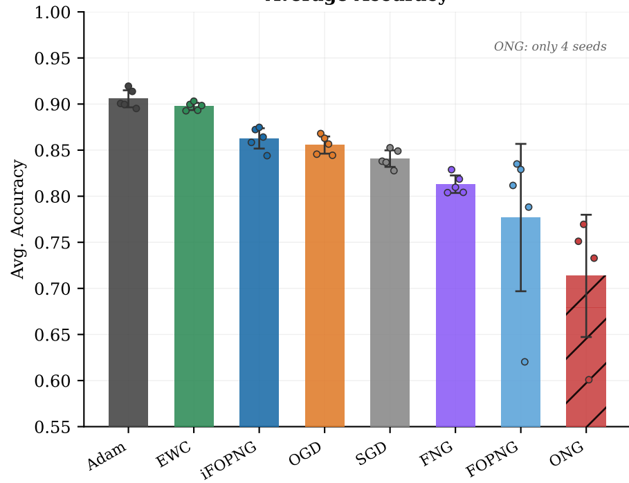
Average Accuracy
