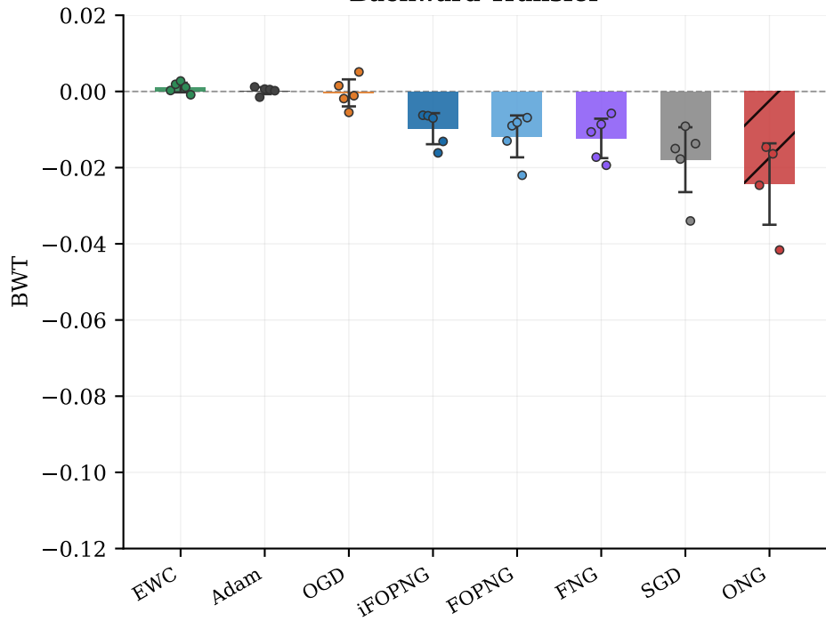
Backward Transfer
