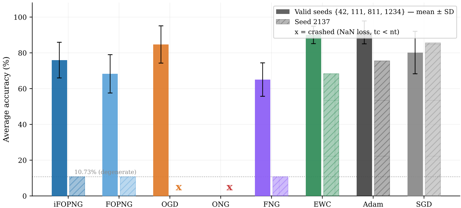
Seed-2137 initialization failure — Split-MNIST HN (Exp. 7)
