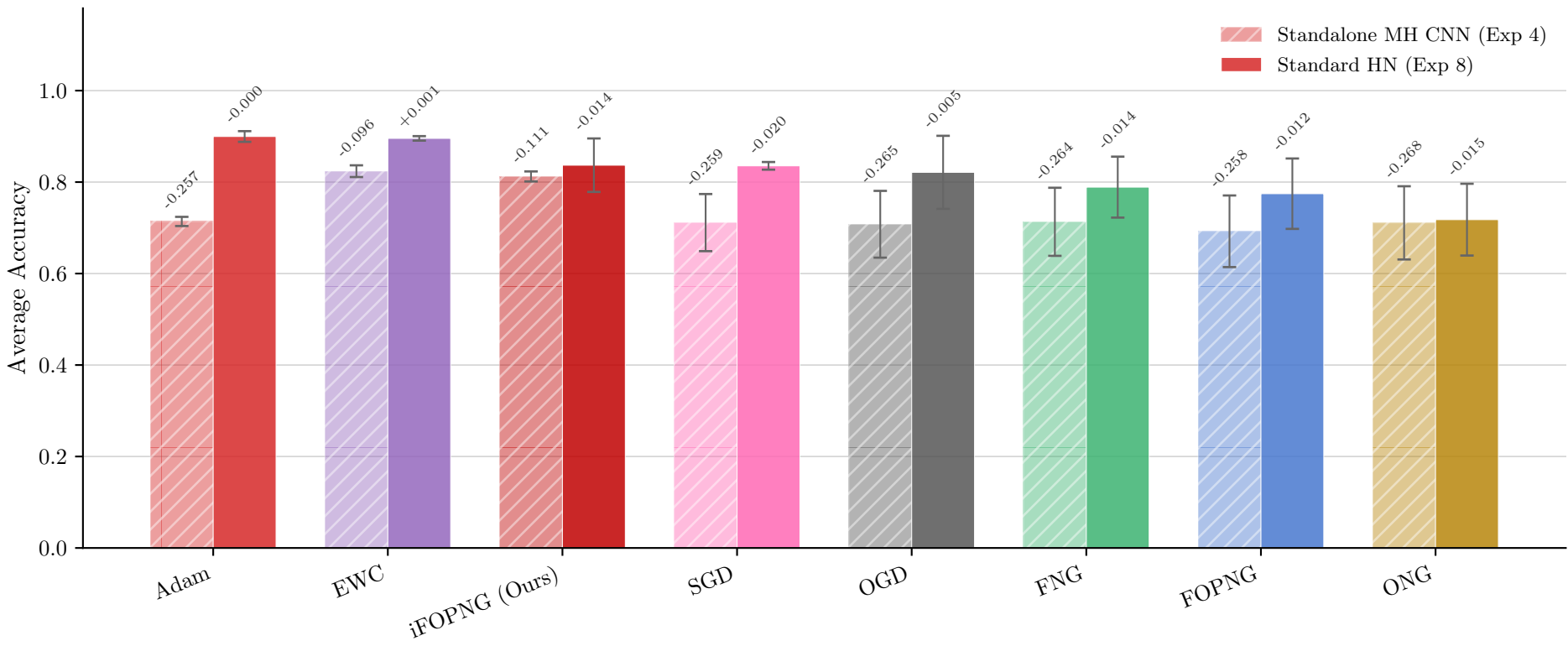
Split-CIFAR10 — Final Average Accuracy (after Task 5)
