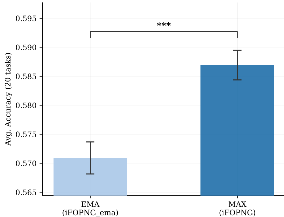
Mean +- std with significance
