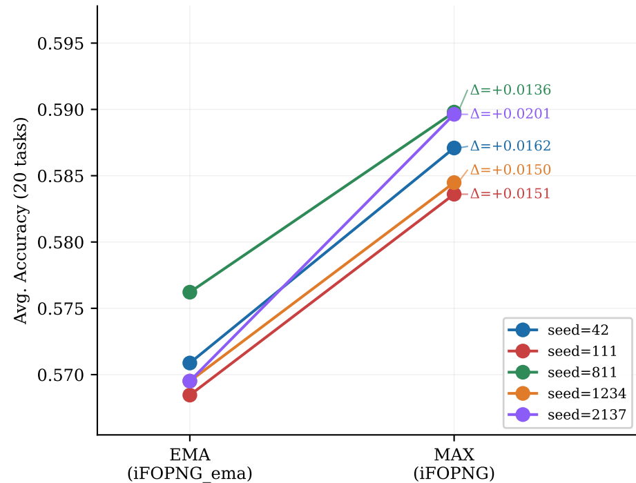
Paired per-seed comparison
