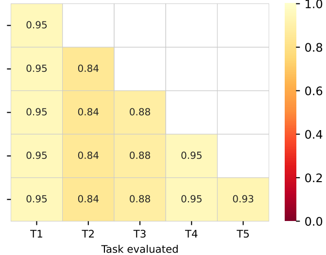
Adam
