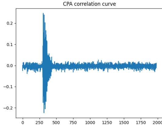
Figure 7: Correlation Power Analysis Curve
