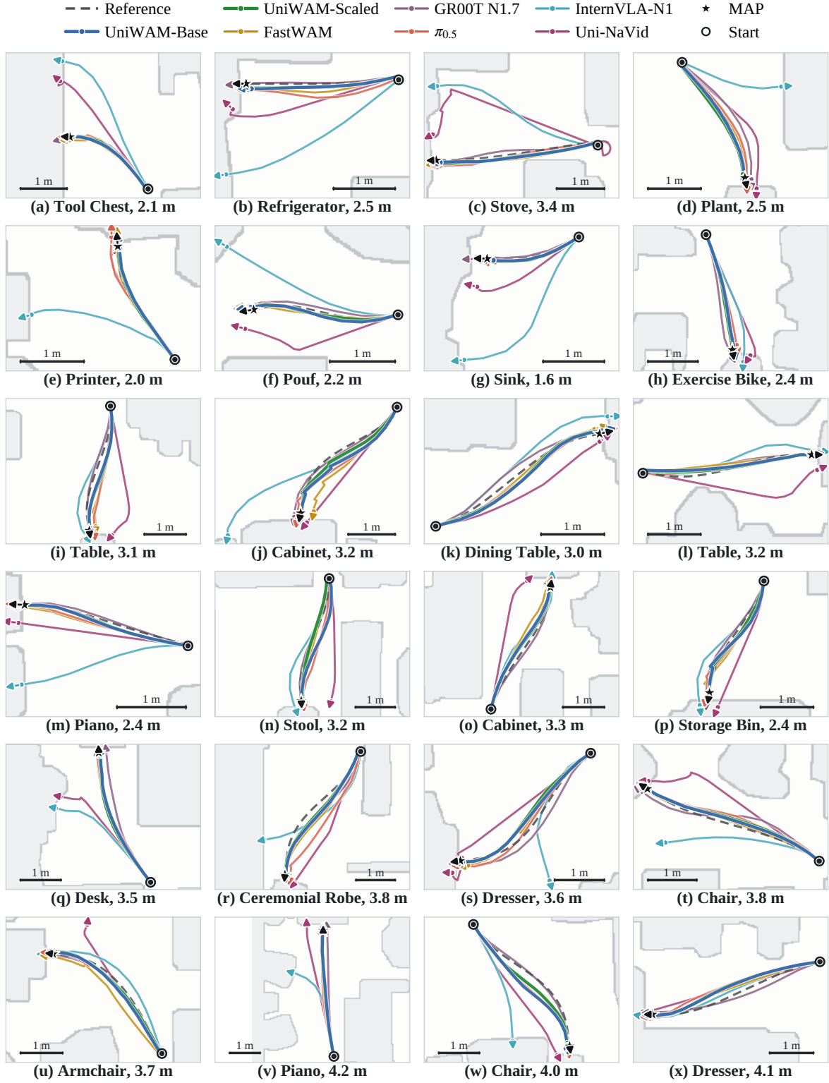
Figure 5 MAP-Bench trajectories of all evaluated methods on 24 randomly selected scenes. Subcaptions give the target category and initial distance. Stars mark the reference MAP, circles the start pose, and arrowheads the terminal heading. In the last two rows, every episode starts at least 3.5 m from the MAP, which falls in the long range.
