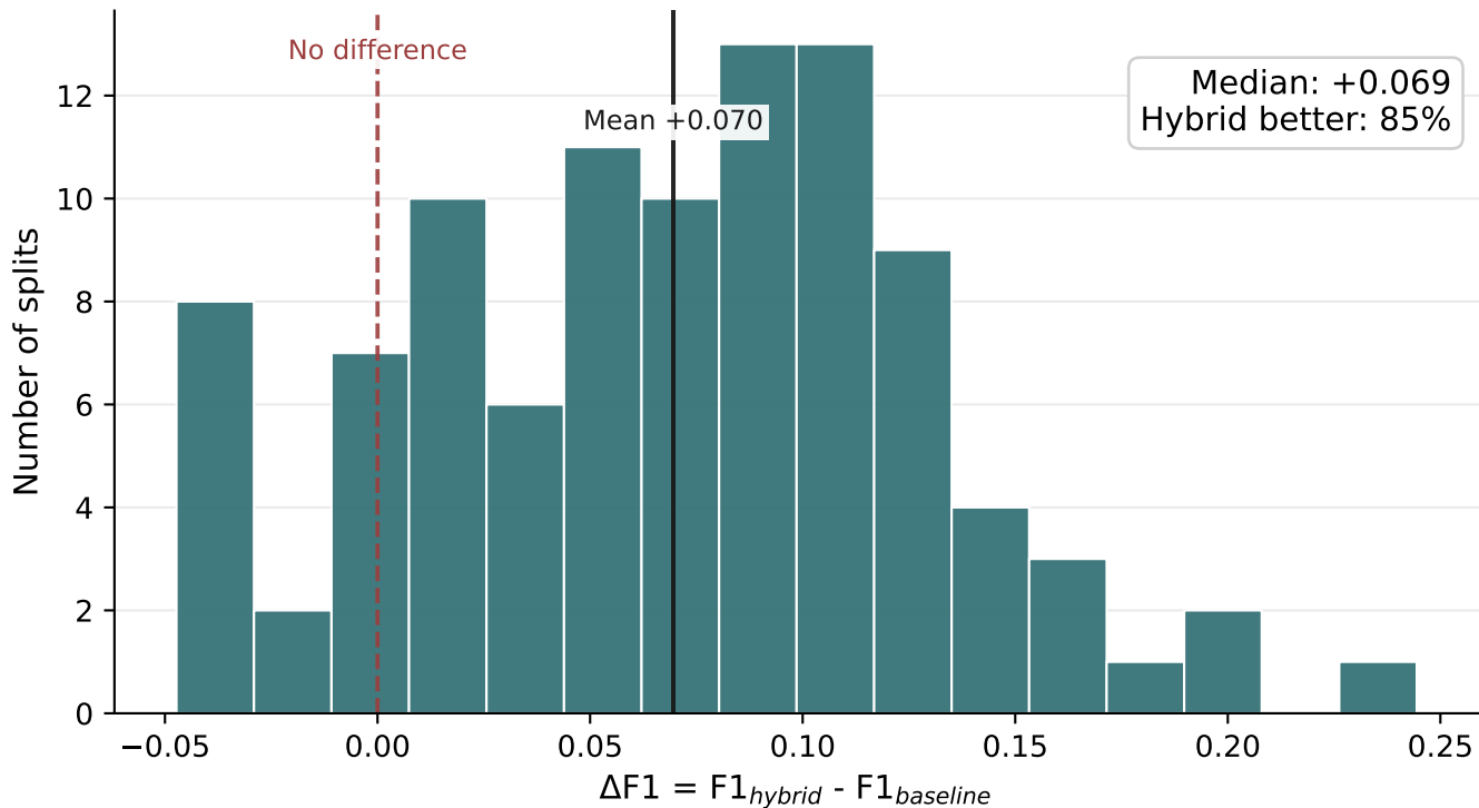
Paired F1 differences across 100 split perturbations
