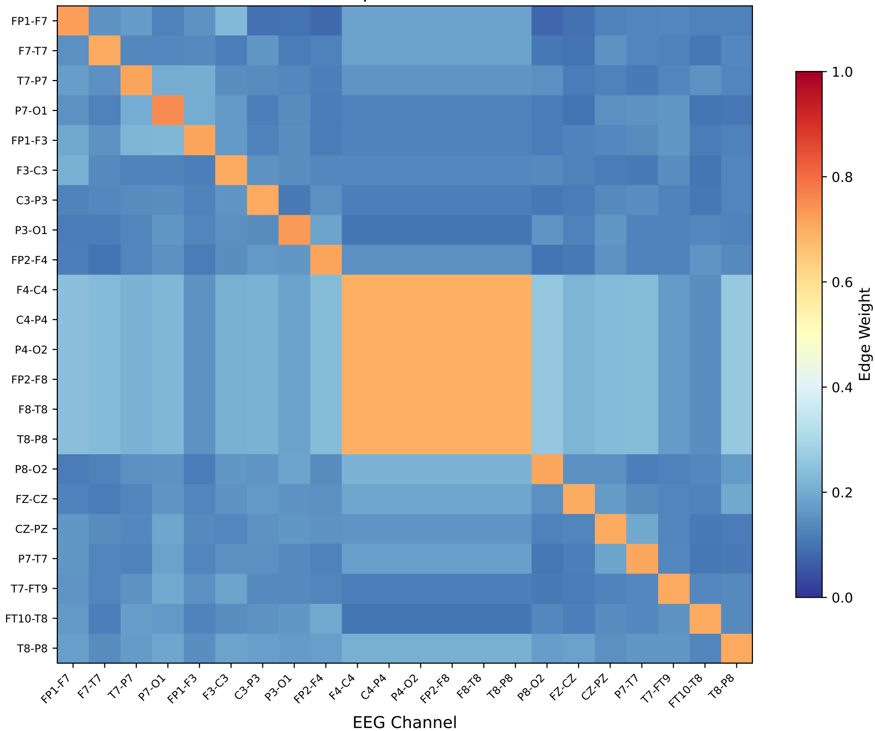
Learned Graph Structure - CHB07
