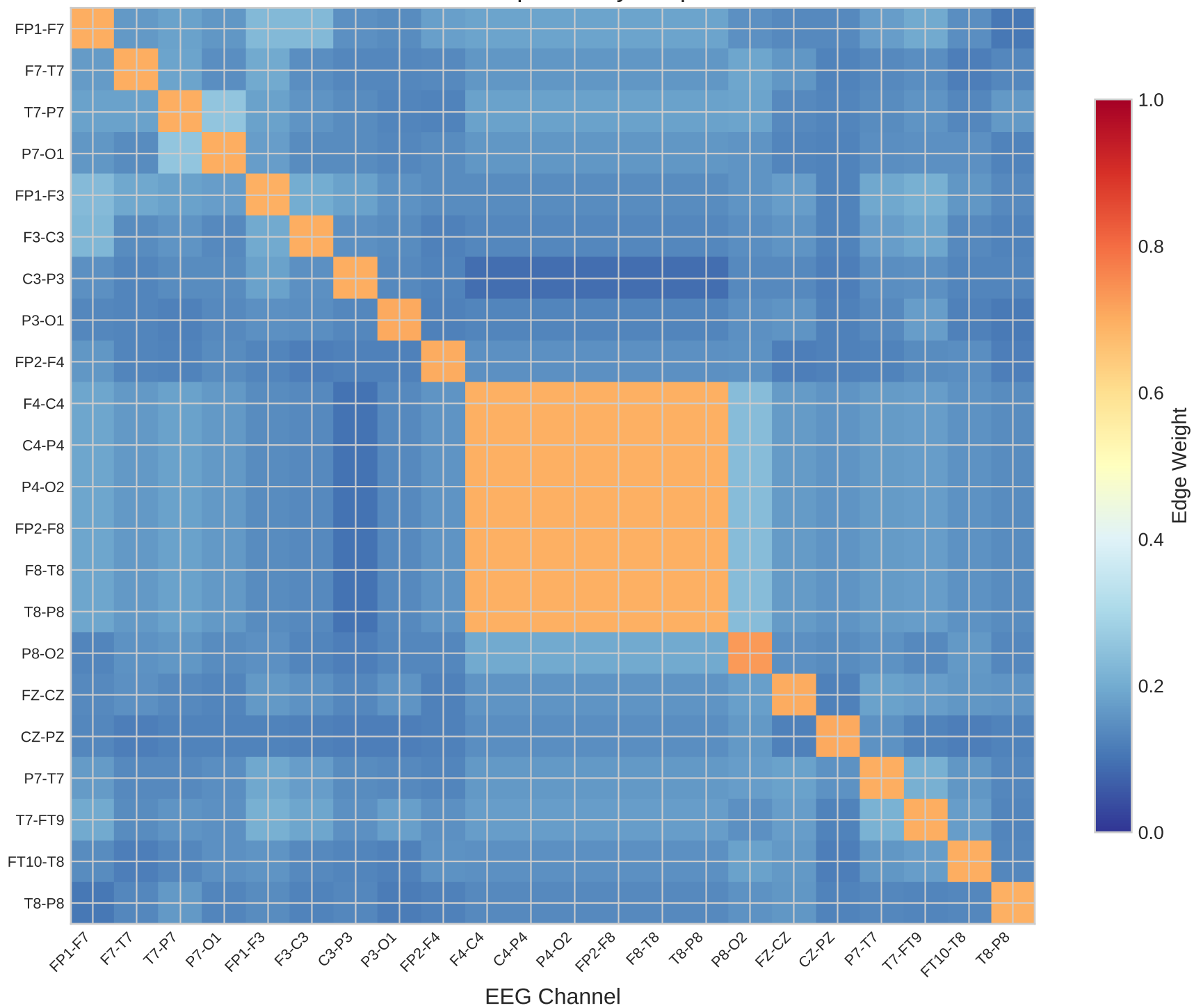
Learned Feature Dependency Graph Structure
