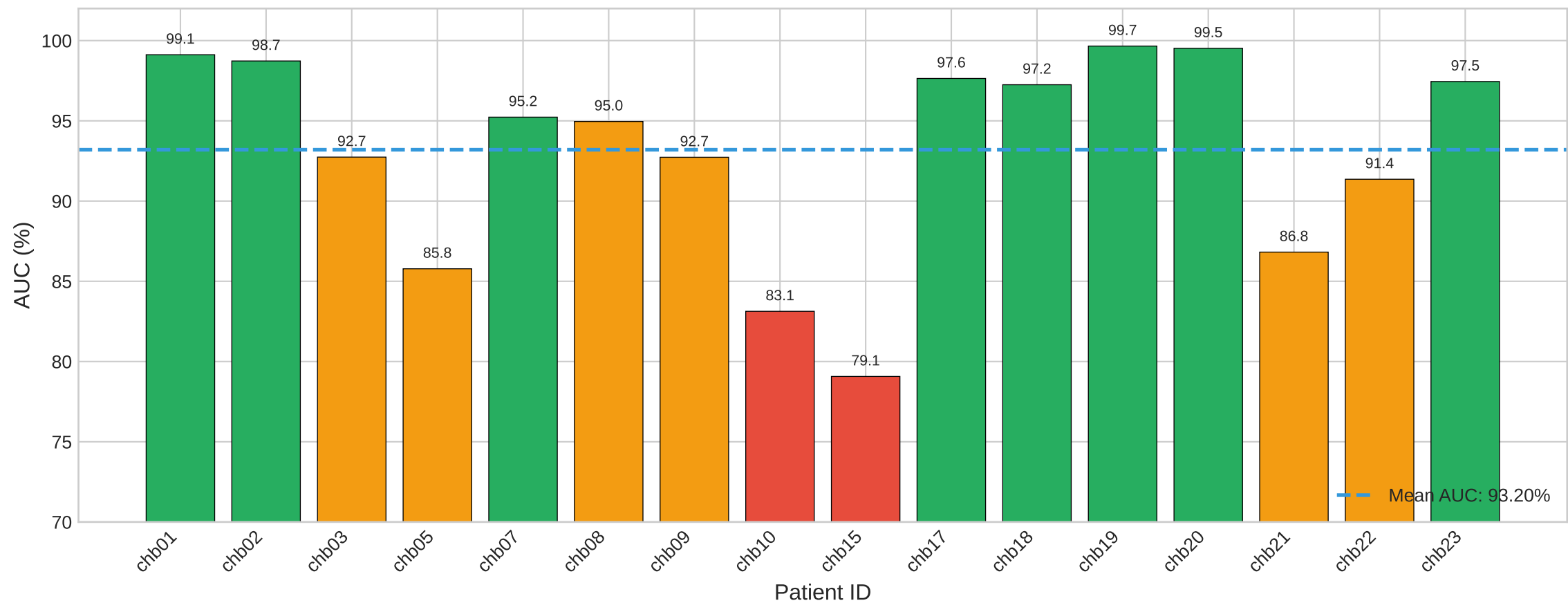
Per-Patient AUC Performance Under LOSO Evaluation
