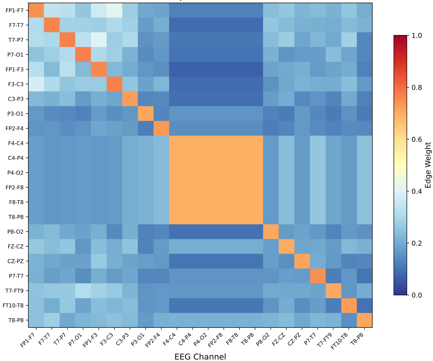
Learned Graph Structure - CHB19
