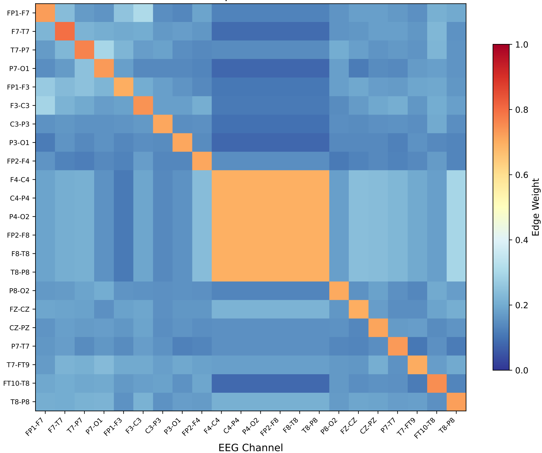
Learned Graph Structure - CHB03
