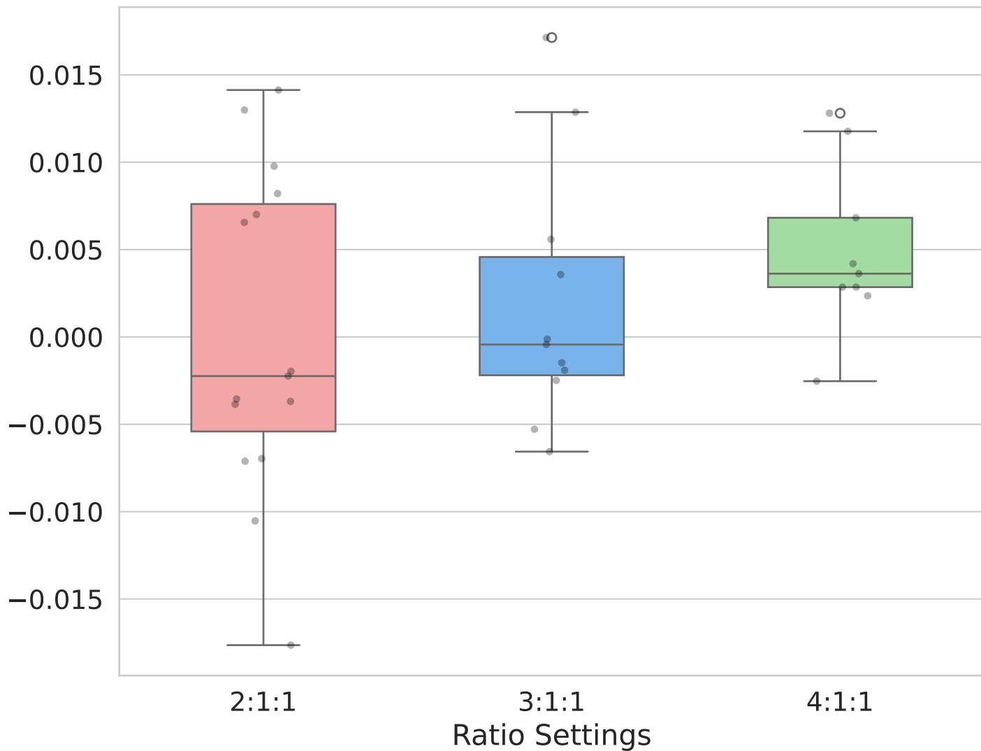
Text-Audio Cosine Similarity
