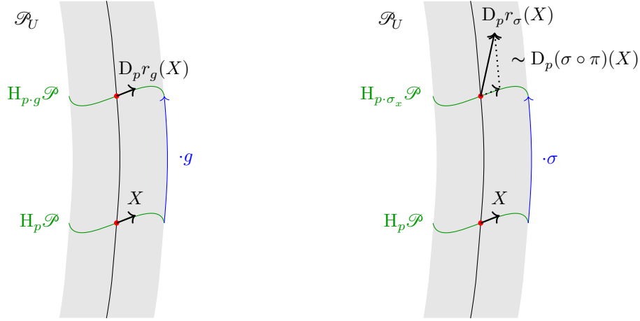
FIGURE 1. Push-forward of a horizontal tangent vector X with constant section (left) and general section (right), where \mathcal{P} is a classical principal bundle as in Example 6.3 equipped with a "typical" connection H\mathcal{P} of principal G -bundles ( G the structural Lie group).
