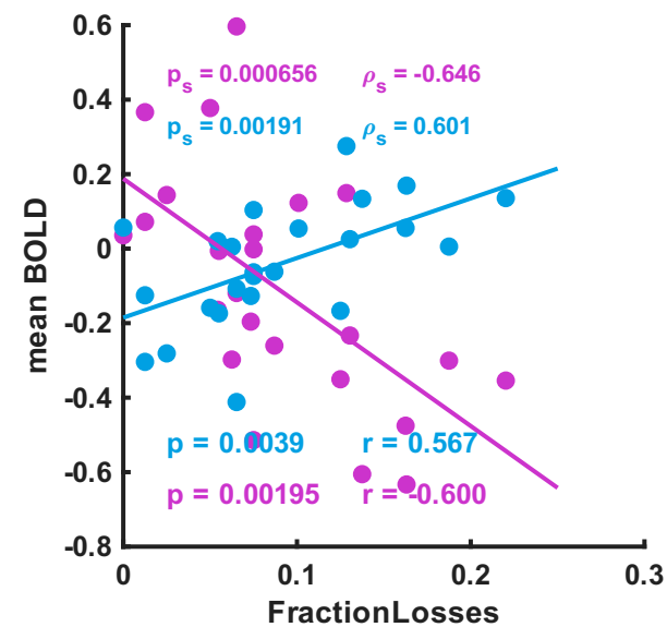
Figure_6D | FractionLosses
