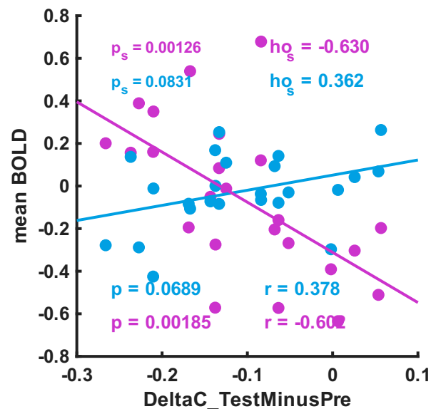
Figure_S13B | DeltaC_TestMinusPre
