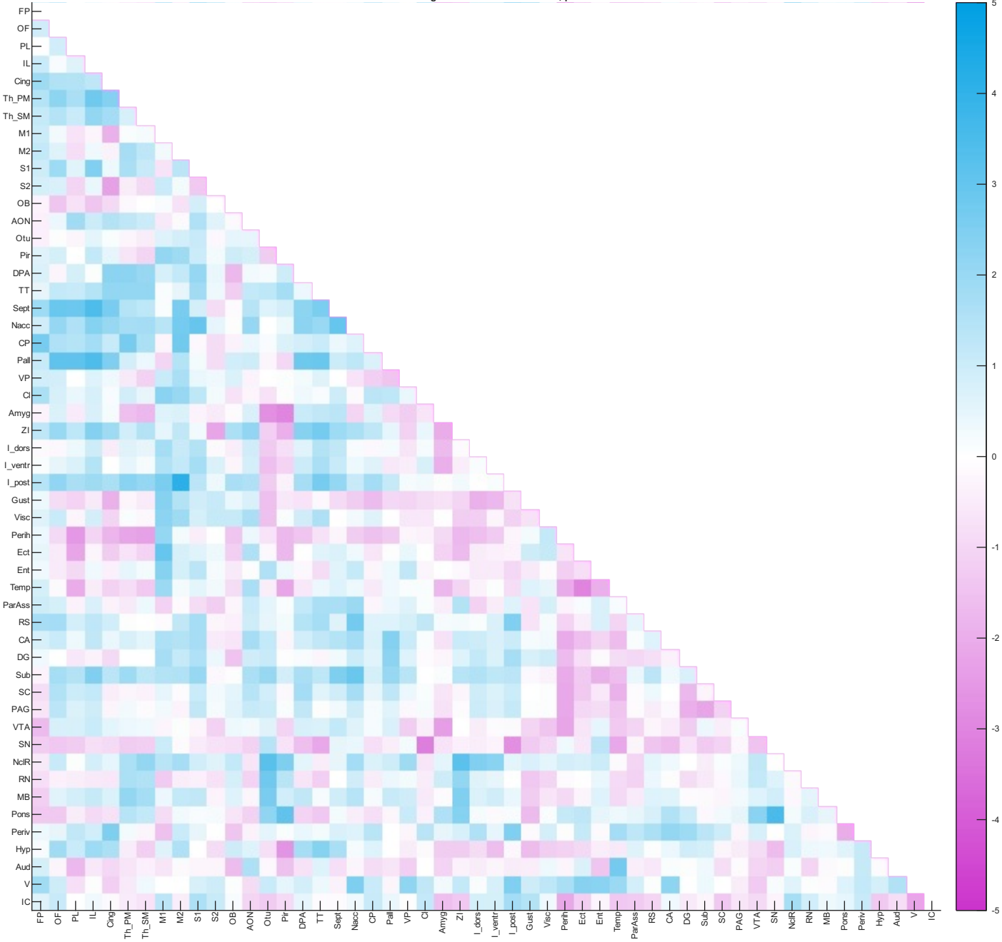
Conditioning cohort: Odor TEST > PRE, paired
