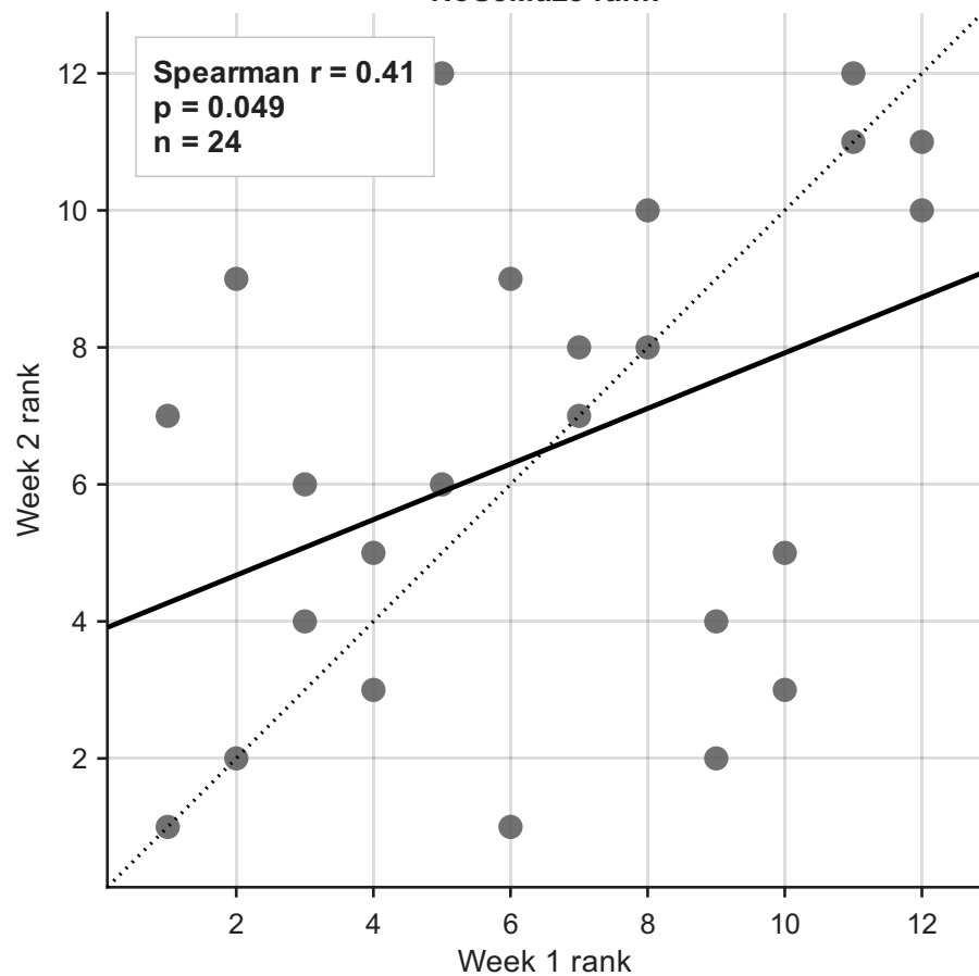
NoSeMaze rank
