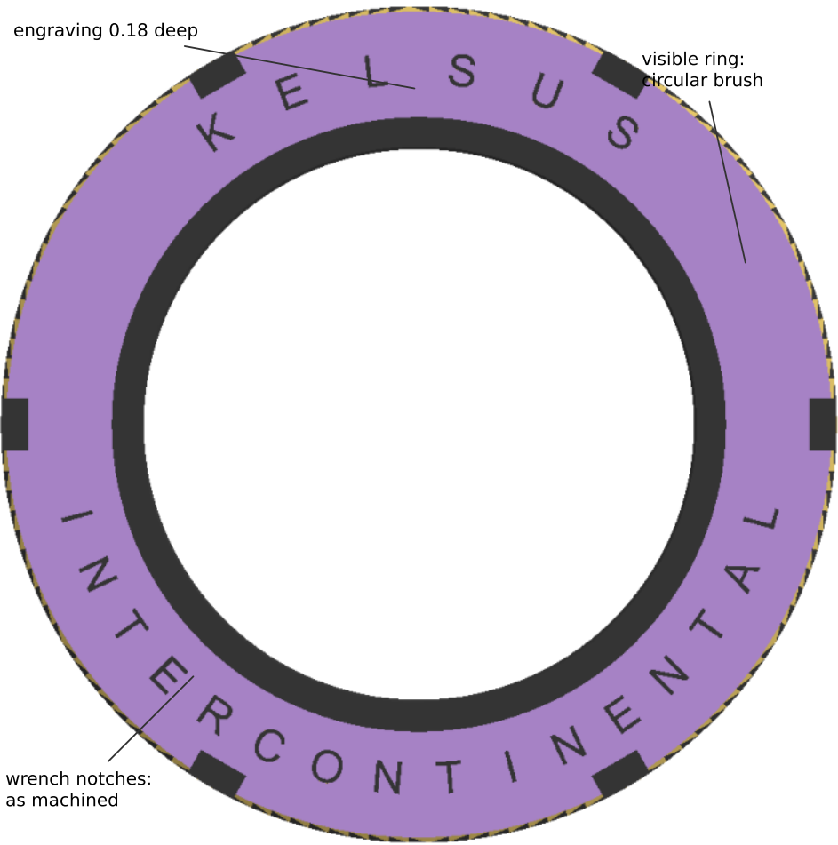
caseback, outside face (as worn view)
