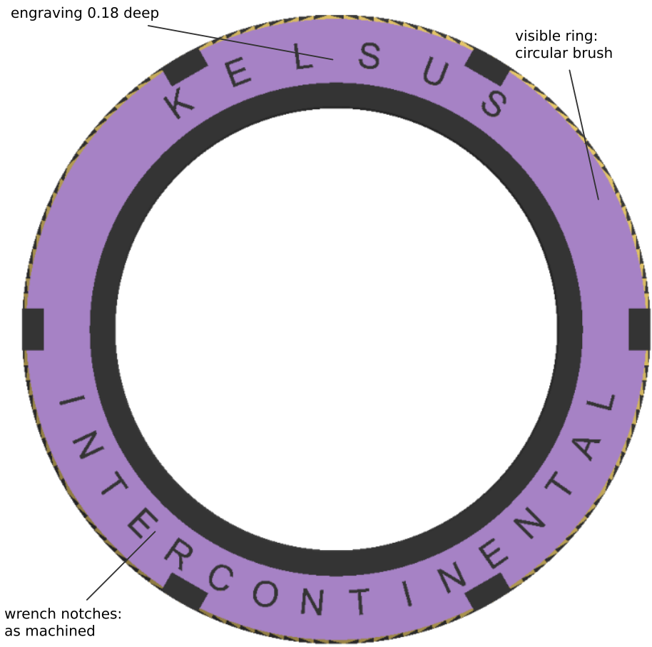
caseback, outside face (as worn view)
