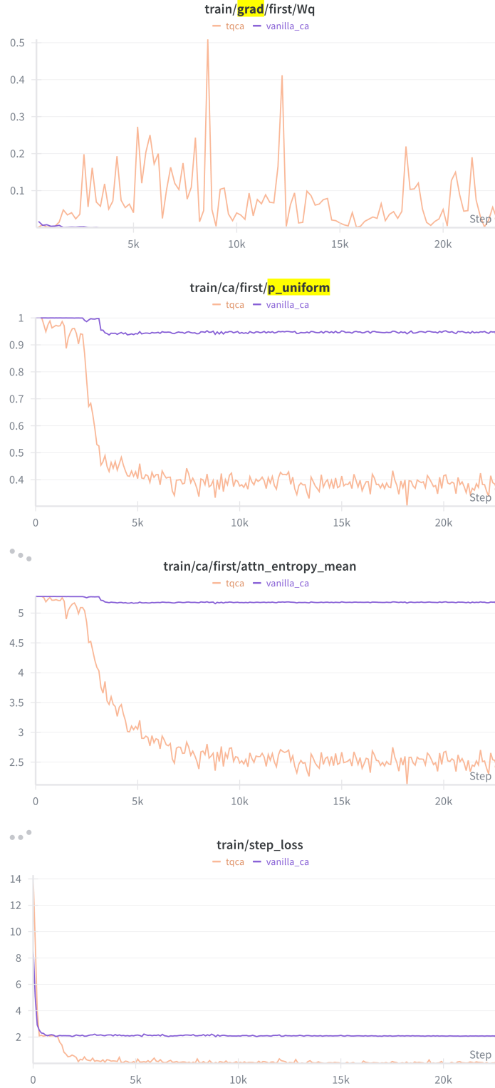
Figure 3: Attention uniformity ( p_{\text{uniform}} ), attention entropy, and training loss over epochs for the CLIP backbone on Flickr30k. TQCA drives attention away from the nearly uniform regime found in the vanilla cross-attention model and achieves stable optimization.
