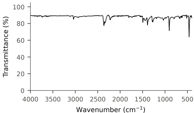
(a) As recorded (ATR, 4\text{ cm}^{-1} )
