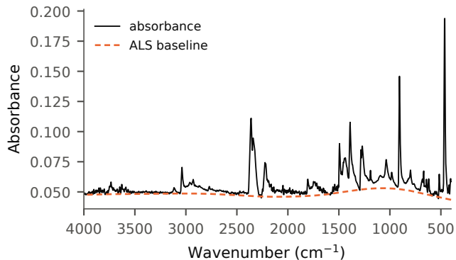
(b) Absorbance and baseline estimate
