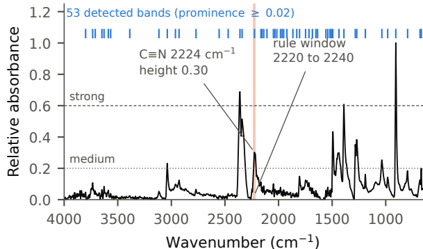
(c) Baseline corrected, normalised, bands detected
