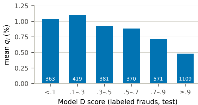
Fig. S2. Mean q_i (%) for test frauds by D score; the values are descriptive, with no interval shown (white numbers are cases per bin). Scores are uncalibrated outputs of a class-reweighted classifier and should not be interpreted as calibrated real-world fraud probabilities.
