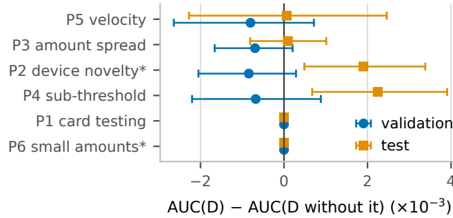
Fig. S1. Exploratory ablation with paired group intervals (* proxy).
