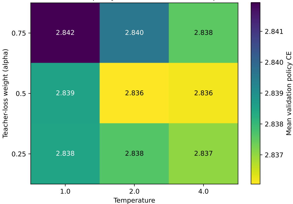
Validation policy loss for distillation sweep
