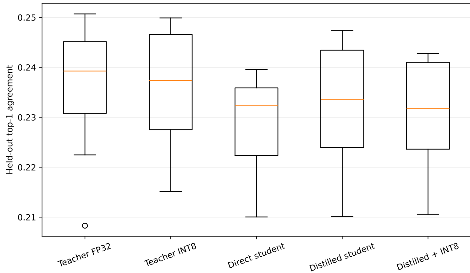
Variation across random seeds
