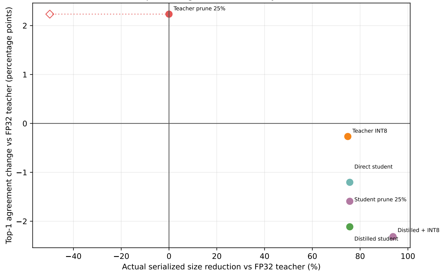
Compression gained vs accuracy retained
