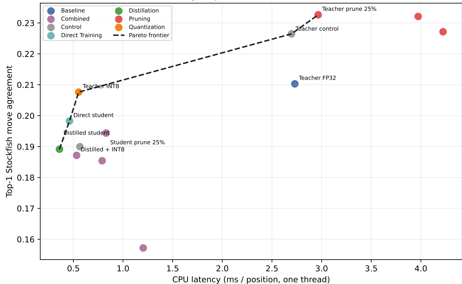
Accuracy vs practical CPU inference cost
