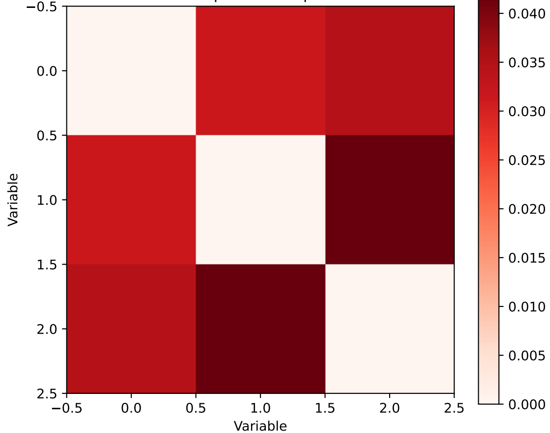
Vine Correlation Error
