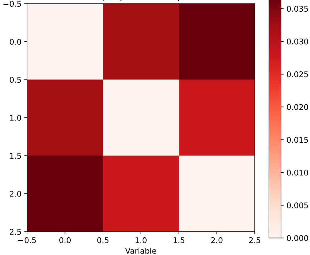
Empirical Correlation Error
