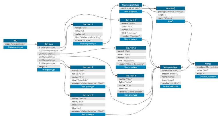
2026-01-22T2234UnifiedModelingLanguage_-_ClassDiagram_-_Creation.png
