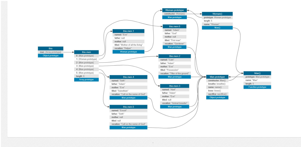
2026-01-22T2234UnifiedModelingLanguage_-_ClassDiagram_-_Creation.png
