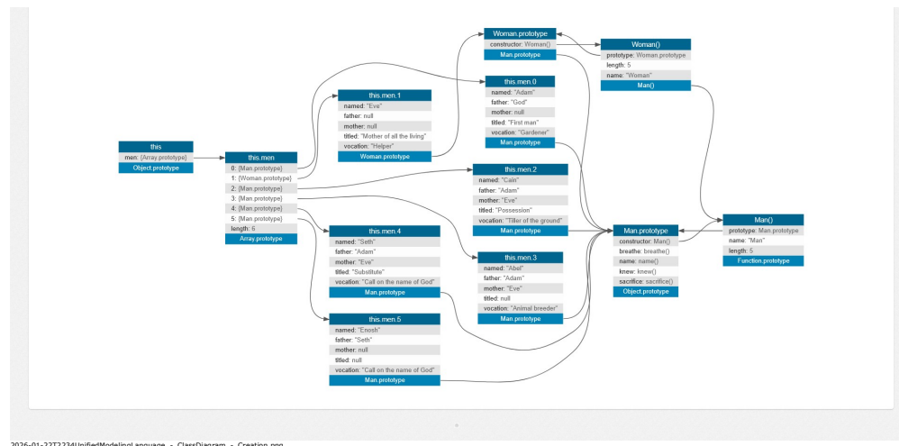
2026-01-22T2234UnifiedModelingLanguage_-_ClassDiagram_-_Creation.png
