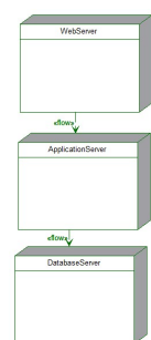
Deployment Diagram
