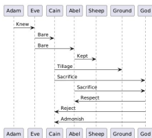
2026-01-25T2155UnifiedModelingLanguage_-_SequenceDiagram_-_CainAndAbel_-_Genesis4.png
