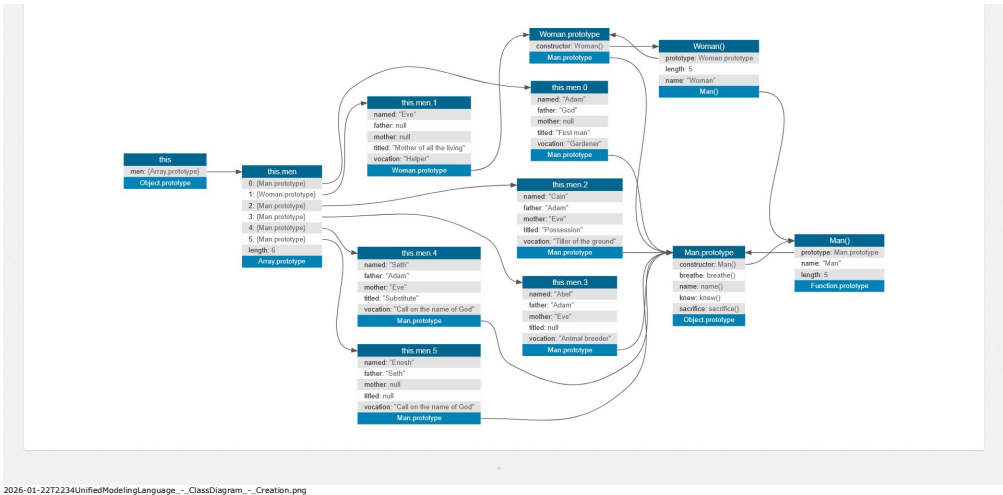
2026-01-22T2234UnifiedModelingLanguage_-_ClassDiagram_-_Creation.png
