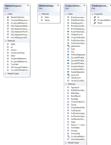
Class Diagram
