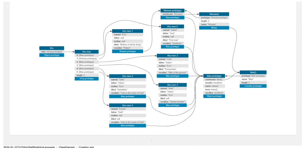
2026-01-22T2234UnifiedModelingLanguage_-_ClassDiagram_-_Creation.png
