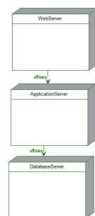
Deployment Diagram
