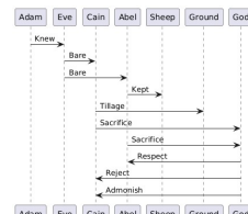
2026-01-25T2155UnifiedModelingLanguage_-_SequenceDiagram_-_CainAndAbel_-_Genesis4.png
