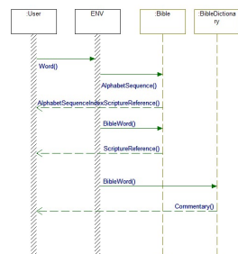
Sequence Diagram
