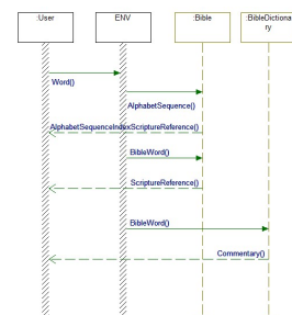
Sequence Diagram
