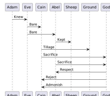
2026-01-25T2155UnifiedModelingLanguage_-_SequenceDiagram_-_CainAndAbel_-_Genesis4.png
