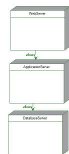
Deployment Diagram
