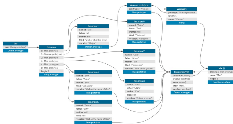
2026-01-22T2234UnifiedModelingLanguage_-_ClassDiagram_-_Creation.png
