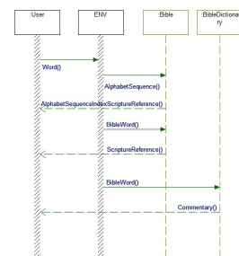
Sequence Diagram
