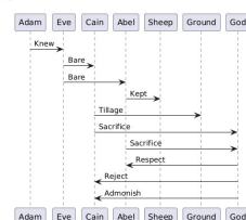
2026-01-25T12155UnifiedModelingLanguage_._SequenceDiagram_._CainAndAbel_._Genesis4.png
