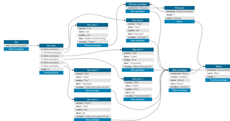
2026-01-22T2234UnifiedModelingLanguage_._ClassDiagram_._Creation.png
