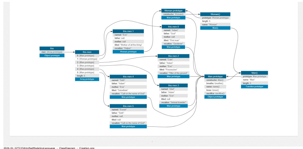
2026-01-22T2234UnifiedModelingLanguage_-_ClassDiagram_-_Creation.png
