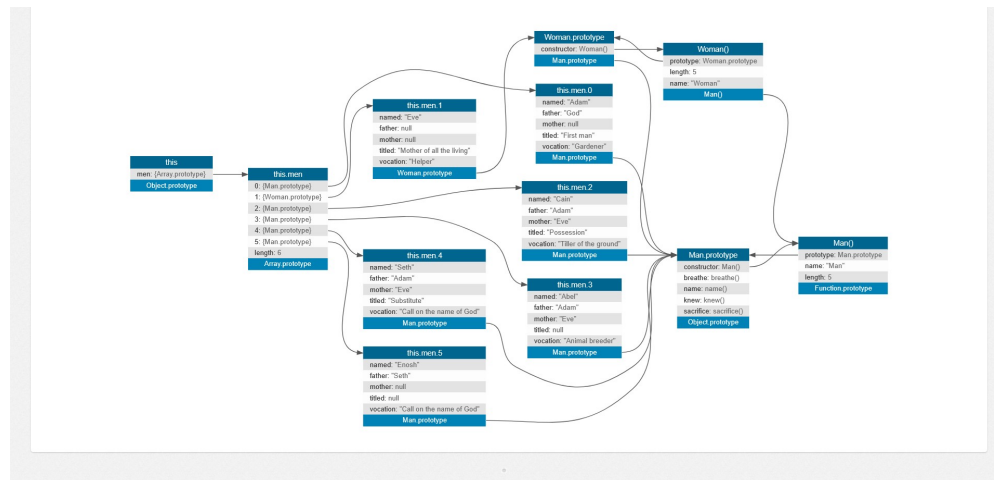
2026-01-22T2234UnifiedModelingLanguage_-_ClassDiagram_-_Creation.png
