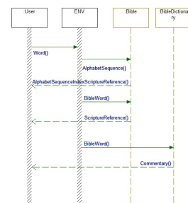
Sequence Diagram
