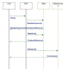
Sequence Diagram
