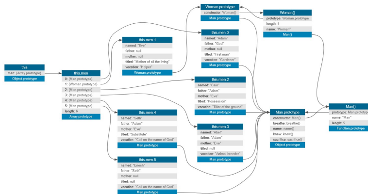
2026-01-22T2234UnifiedModelingLanguage_-_ClassDiagram_-_Creation.png
