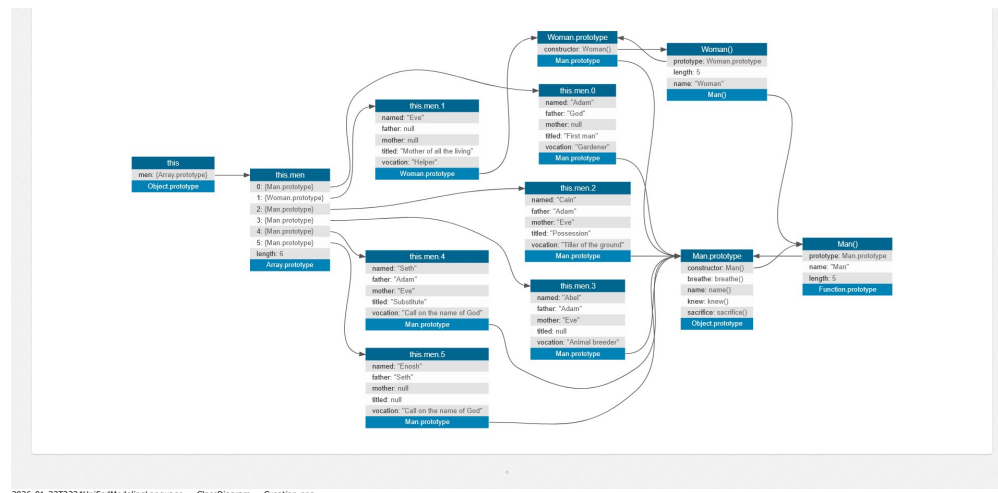
2026-01-22T2234UnifiedModelingLanguage_-_ClassDiagram_-_Creation.png
