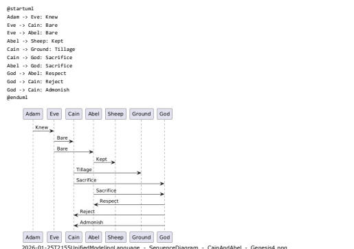
2026-01-2572155UnifiedModelingLanguage_-_SequenceDiagram_-_CainAndAbel_-_Genesis4.png
