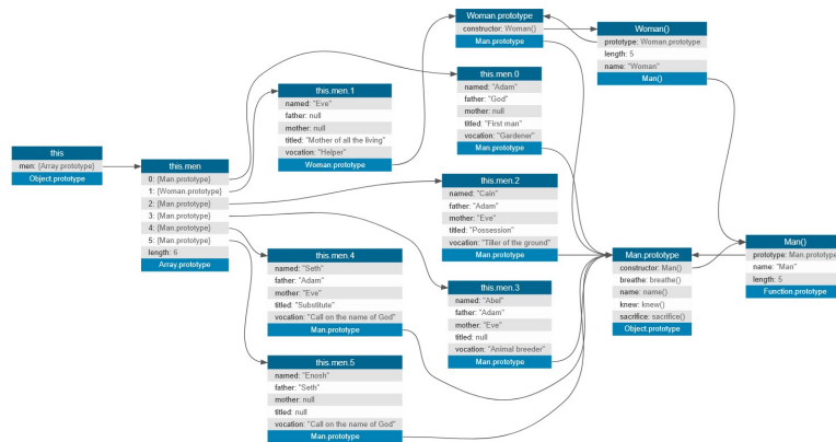
2026-01-227224UnifiedModelingLanguage_-_ClassDiagram_-_Creation.png
