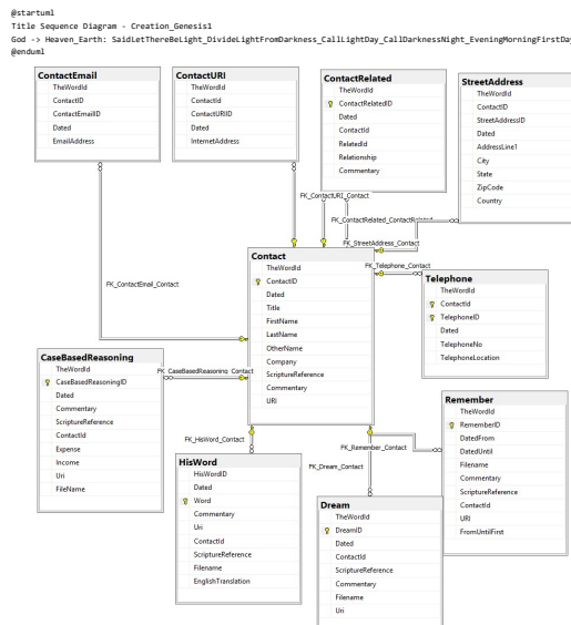
Entity-Relationship Model - Contact
