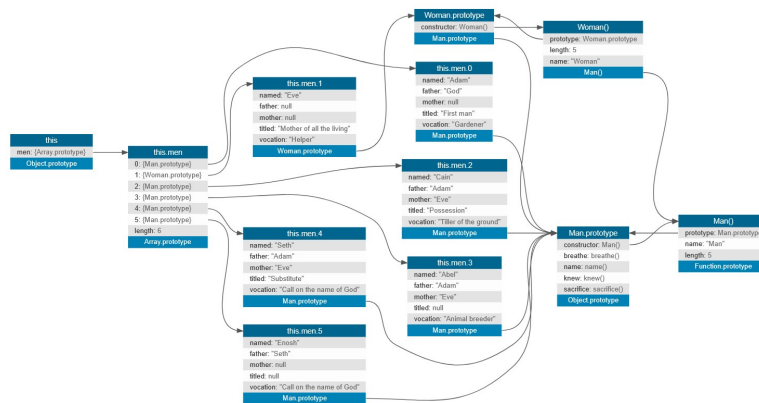
2026-01-22T224UnifiedModelingLanguage_-_ClassDiagram_-_Creation.png
