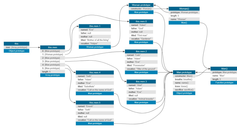
2026-01-22T2234UnifiedModelingLanguage_-_ClassDiagram_-_Creation.png
