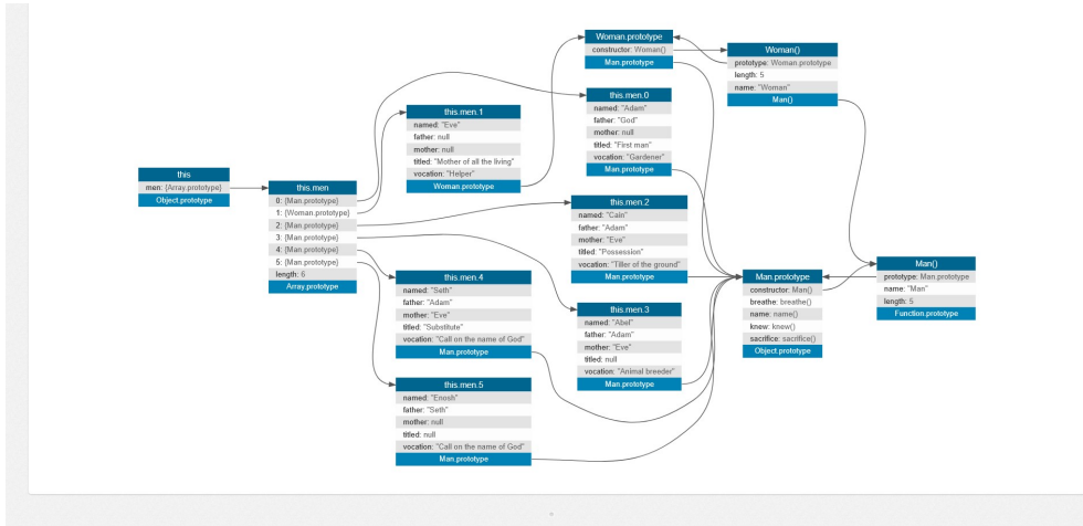
2026-01-22T2234UnifiedModelingLanguage_-_ClassDiagram_-_Creation.png
