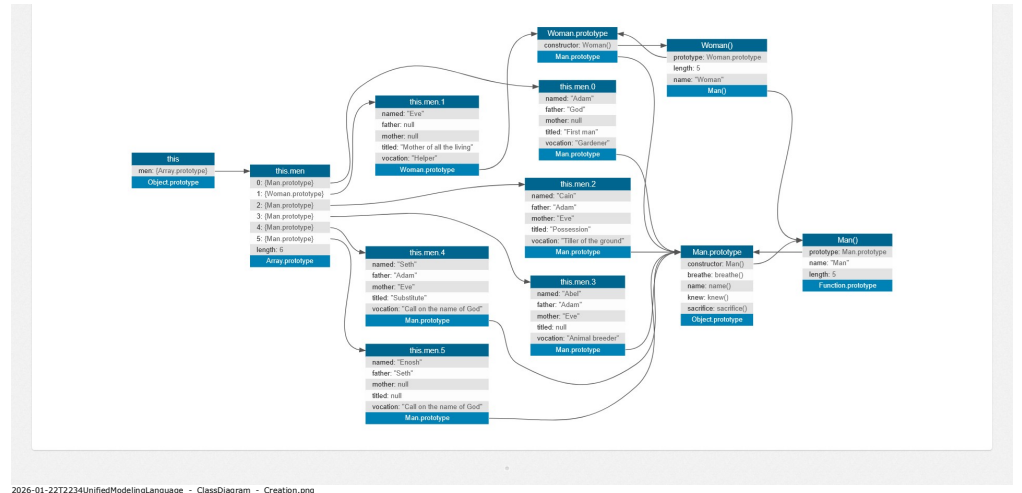
2026-01-22T2234UnifiedModelingLanguage_-_ClassDiagram_-_Creation.png
