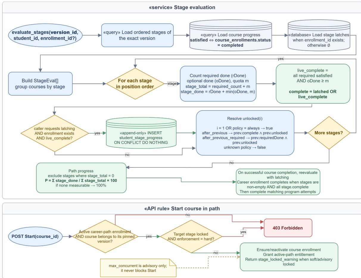
Figure F.2: Career pathway stage evaluation: from pinned version to per-stage completion, unlock, and overall progress.
