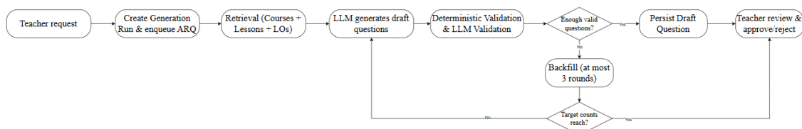
Figure 6.2: Interview Question Generation Pipeline.
