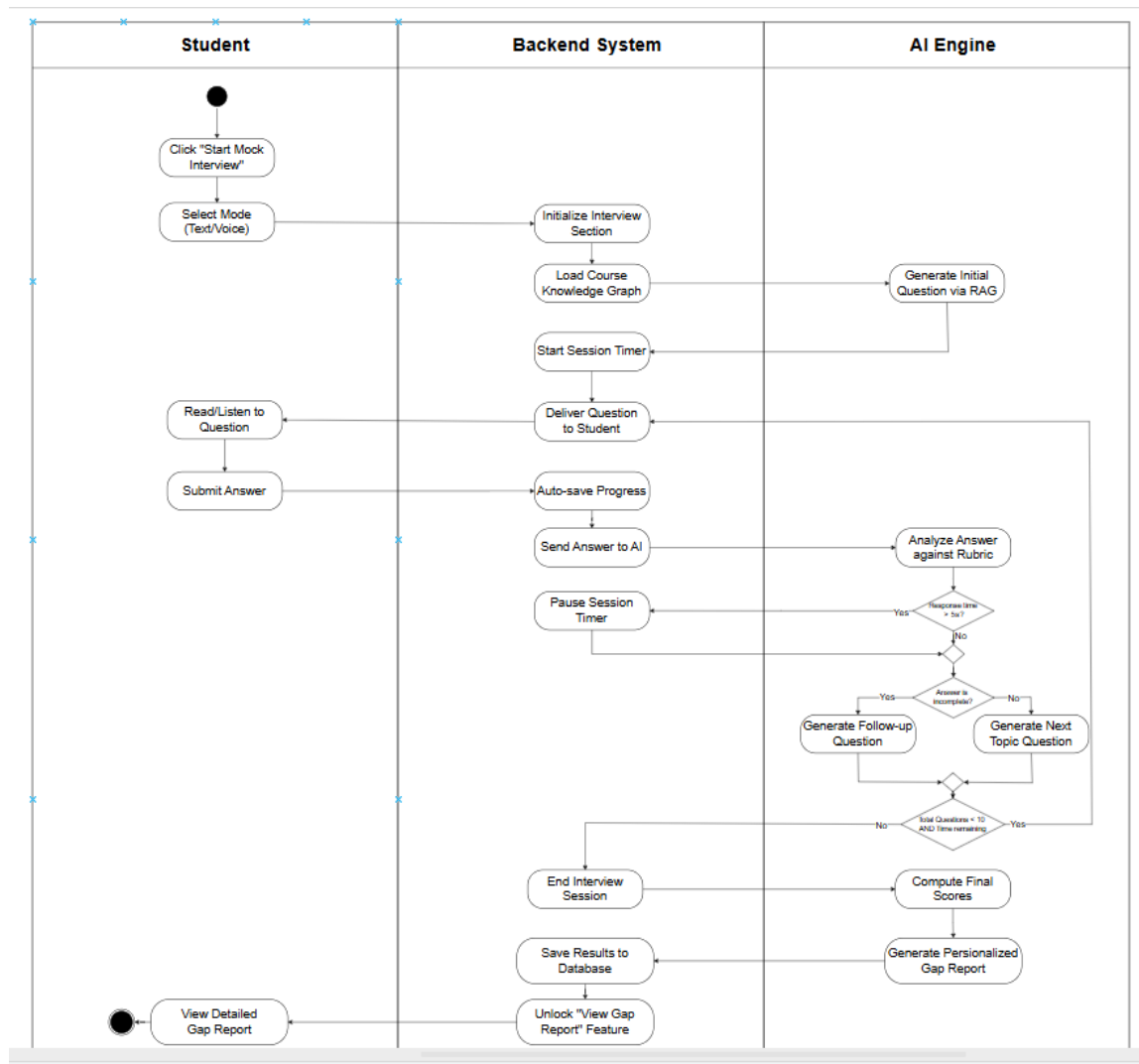
Figure H.4: Activity Diagram: Context-Aware Mock Interview
