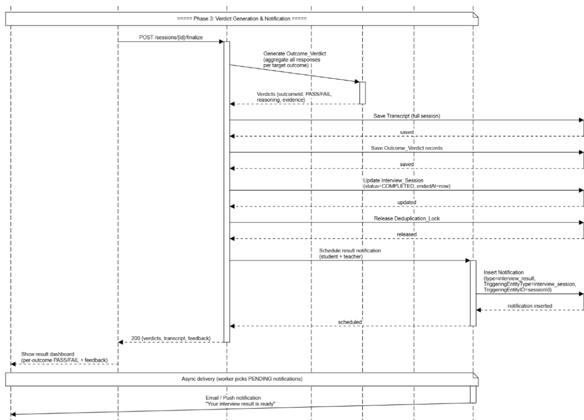
Figure I.6: Sequence Diagram: Mock Interview (Phase 3)
