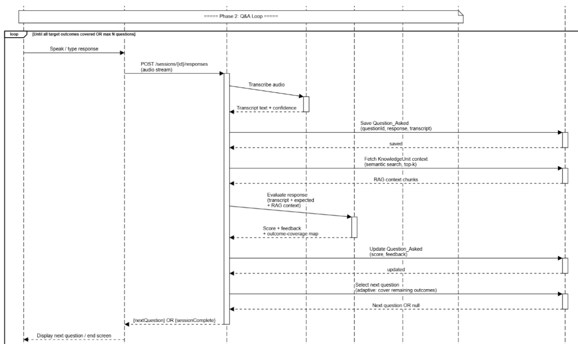
Figure I.5: Sequence Diagram: Mock Interview (Phase 2)
