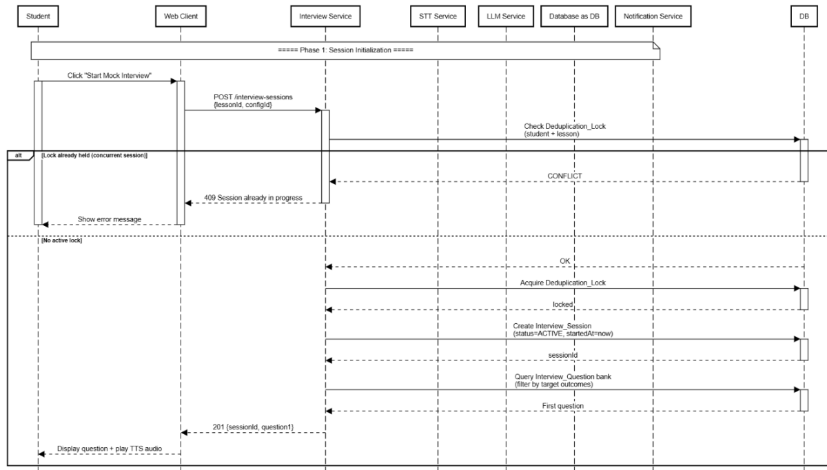
Figure I.4: Sequence Diagram: Mock Interview (Phase 1)
