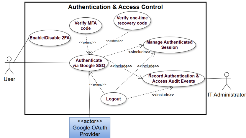
Figure 4.2: Detailed Use Case Diagram: Authentication and Access Control Module
