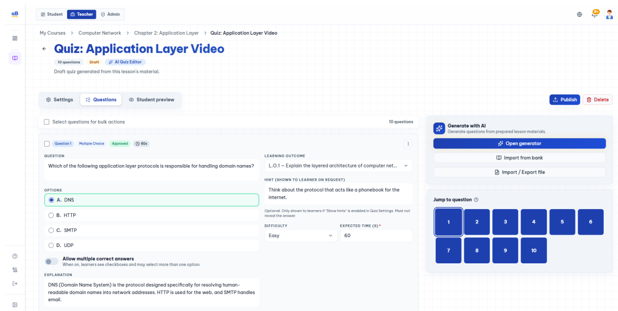
Figure M.10: Quiz Editor — Question list with bulk timing controls and an AI-generation side panel.
