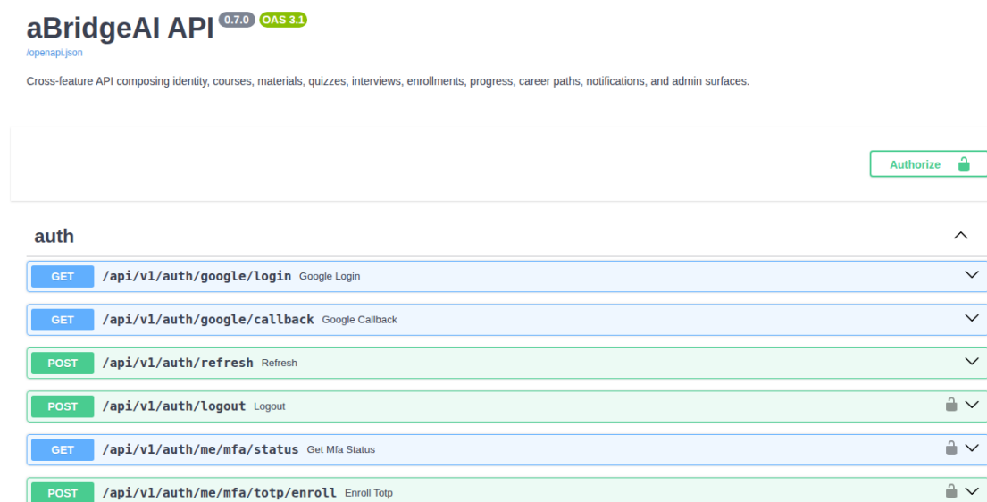
Figure K.1: Live Swagger UI at /docs (rendered from the FastAPI /openapi.json ): title, authorise control, and the auth audience-tag section.
