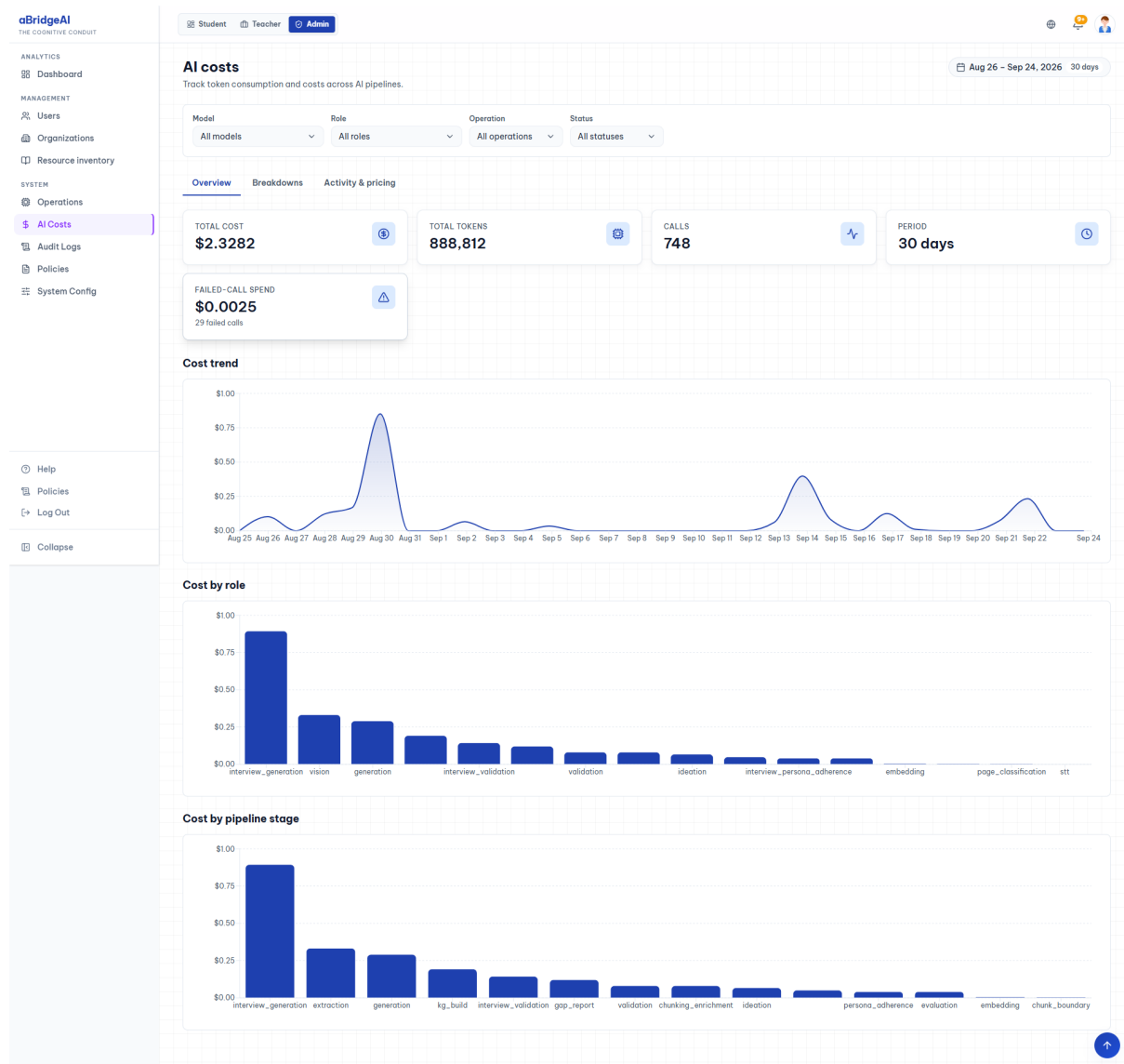
Figure M.14: Admin AI Costs — Token consumption and spend across pipeline roles and stages.
