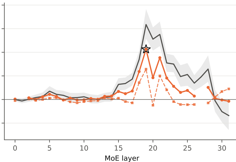
strict set (n_val=128, threshold 64)
