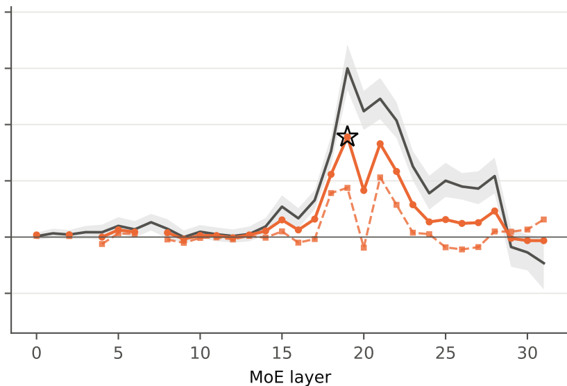
relaxed set (n_val=256, threshold 128)
