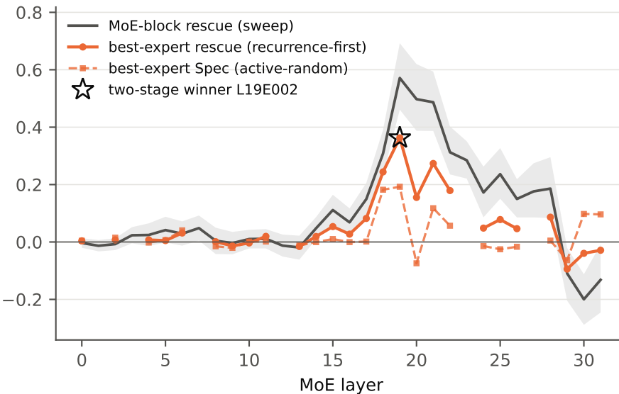
paper set (n_val=128, threshold 64)
