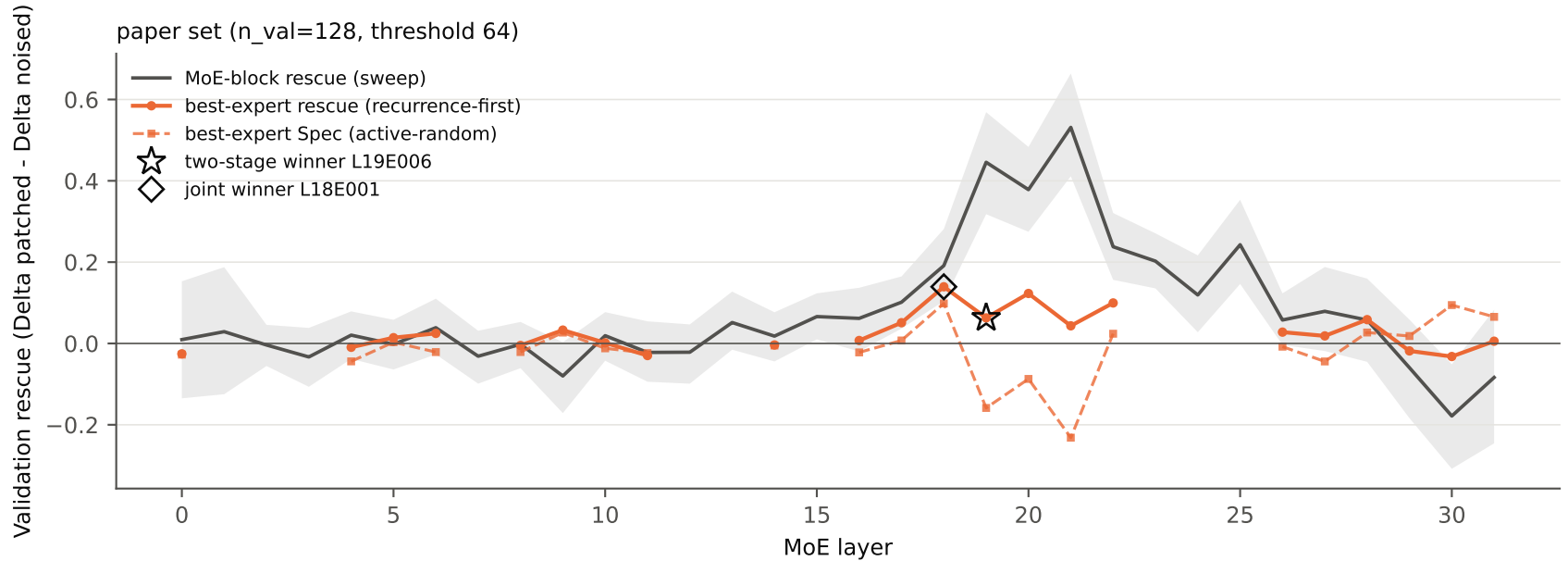
Mixtral-8x7B-v0.1 (no BOS, paper protocol): MoE-block rescue vs best single expert per layer (validation means; 95% band for the block)
