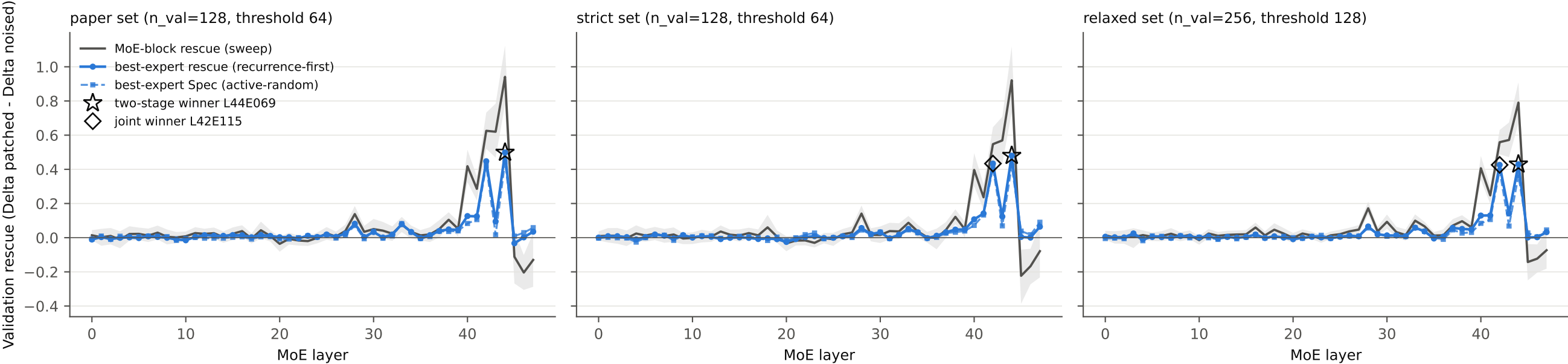
Qwen3-30B-A3B-Base (tokenizer defaults): MoE-block rescue vs best single expert per layer (validation means; 95% band for the block)
