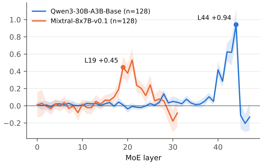
(a) MoE-block output patching across layers
