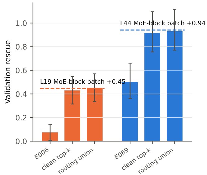
(c) Coalition patching vs MoE-block patch
